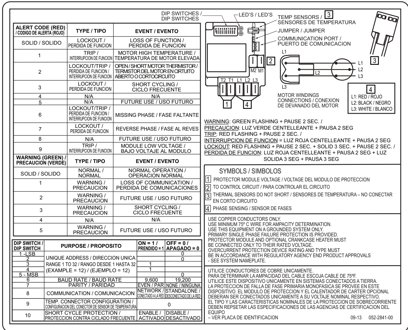
Figure 3 Compressor Terminal Box Wiring with CoreSense Protection
