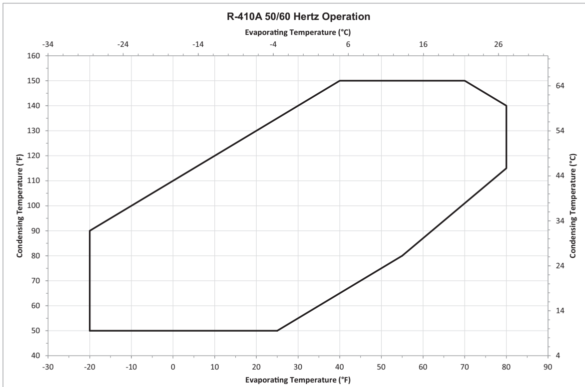
Figure 2 – Scroll Operating Envelopes
